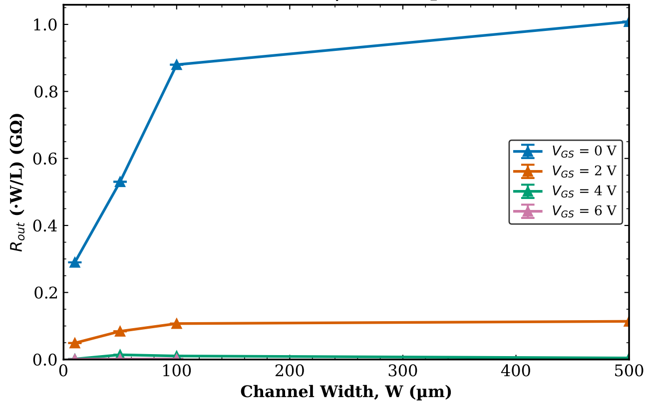
TFT2 Transistor 1 R_{out} vs W | L = 80\text{ }\mu\text{m}
